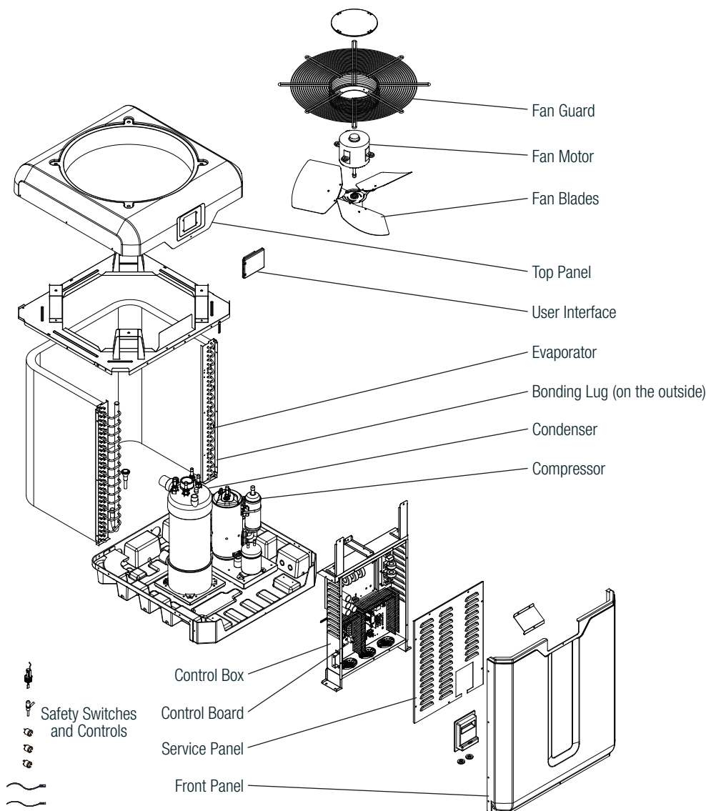
Figure 1 : Name of Heat Pump Components
