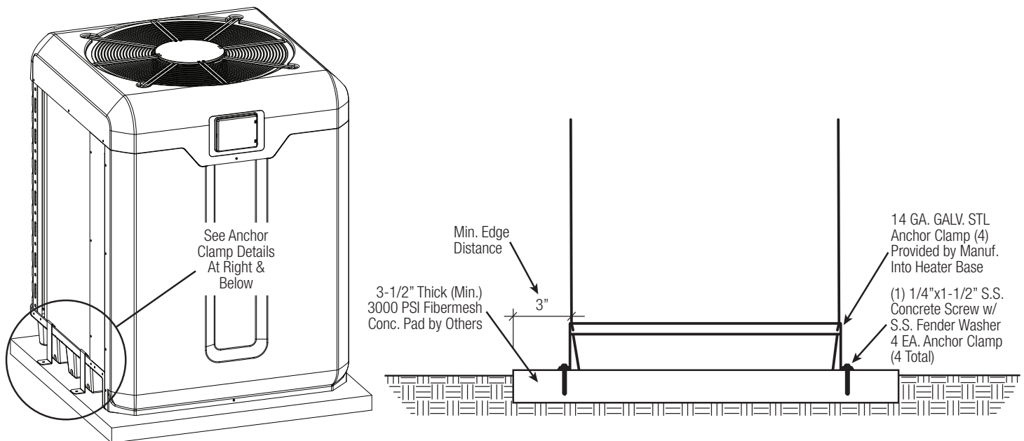
Figure 4: Equipment Pad and Anchoring
