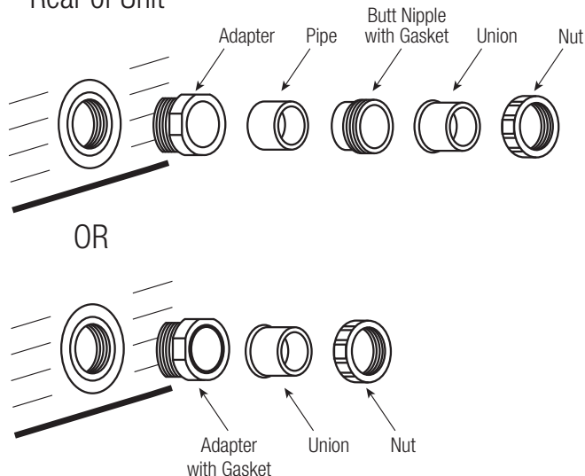
Figure 6: In Ground Included Connectors Rear of Unit
