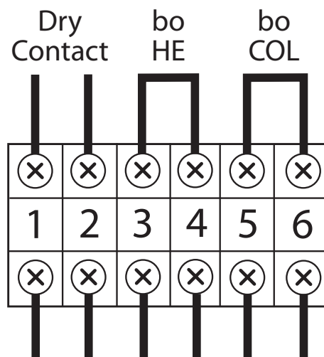
Figure 11: Remote ON/OFF
