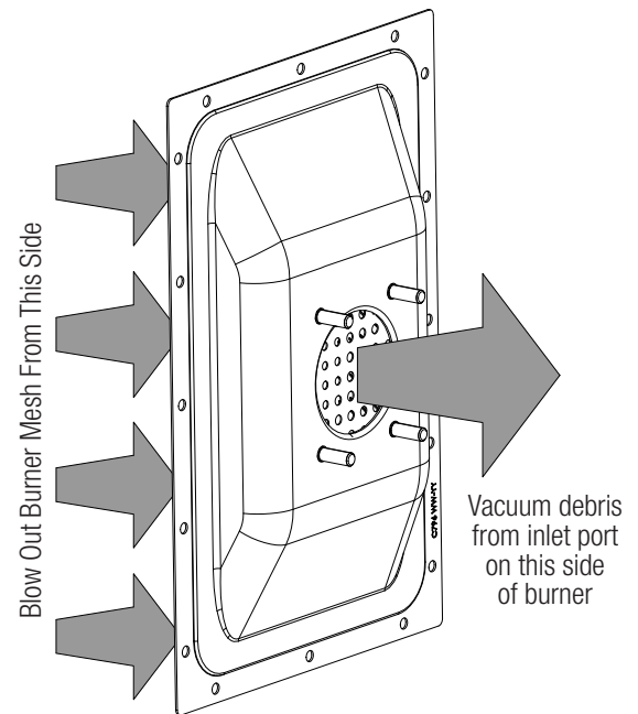
Figure 24: Burner Cleanout
