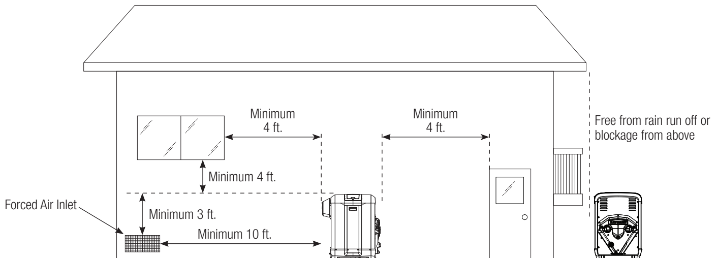
Figure 4: Outdoor Minimum Clearances
