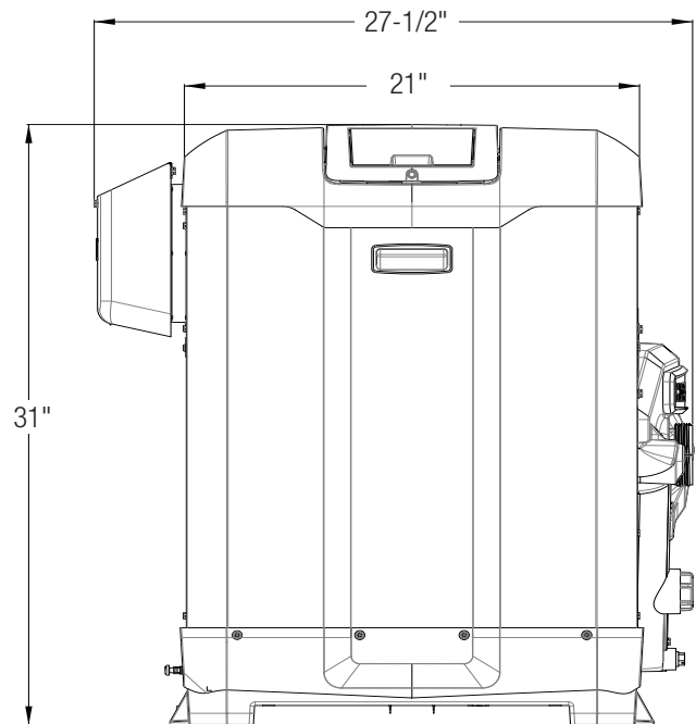
Figure 2: Heater Dimensions
