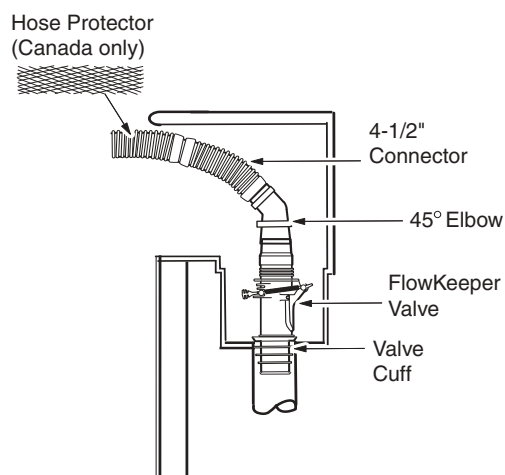
Skimmer Installation
