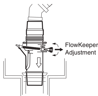
Skimmer Installation
