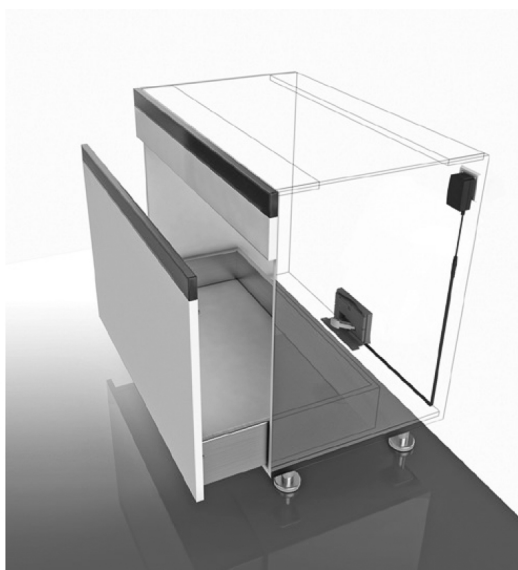
Spacer pin installed on the drawer. Spring-loaded spacer pins are used on adjacent doors to ensure the same clearance from the unit frame.
