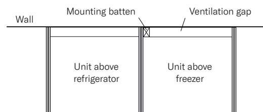
Placement of mounting batten for wall units above refrigerators and freezers.
