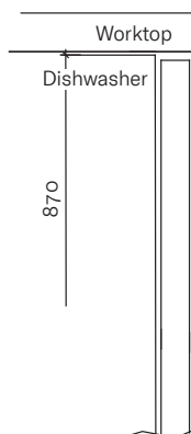
H series with tall appliance.
