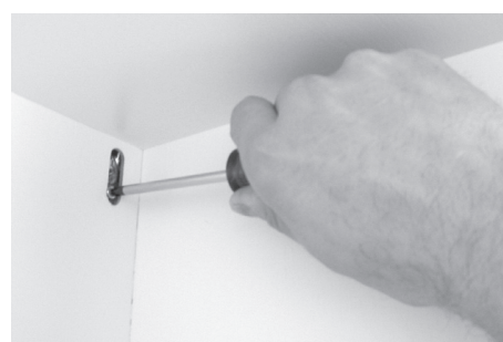
The hanging bracket is easily adjusted with a standard screwdriver. Cover this hole with the cover cap after making the adjustment.
