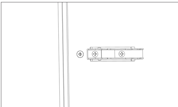
Suitable placement of assembly screws. Once the door is mounted, the hinge will cover the screw head.
