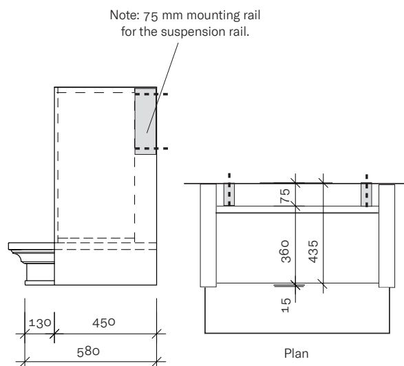
Detail view of the Sundby extractor hood.
