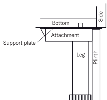
Plinth leg assembled under unit. The legs are positioned under the unit joint to absorb as much of the load as possible.
