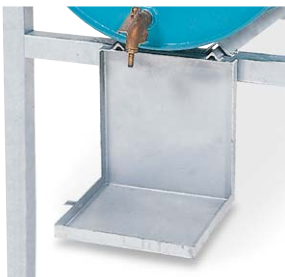
Steel dispensing tray, galvanised Dimensions W x D x H: 280 x 270 x 300 mm Order number: 114-543-M2
