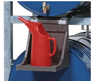
Dispensing tray in polyethylene (PE) Dimensions W x D x H: 270 x 270 x 300 mm Order number: 114-902-M2
