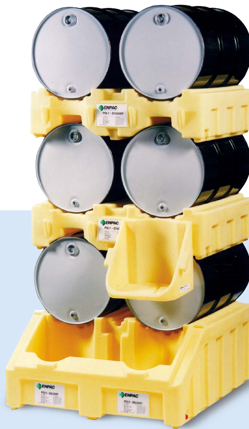
Image shows a Drum Racker together with two optional Stacker and a Dispensing Shelf
