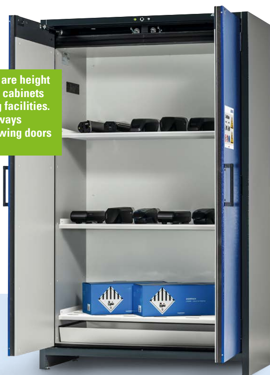
Battery Cabinets - Fire-Rated - wide model - with 3 shelves Order no. M31-8083-U2
