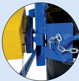
Safety first - a chain fixed the drum onto the Stacker
