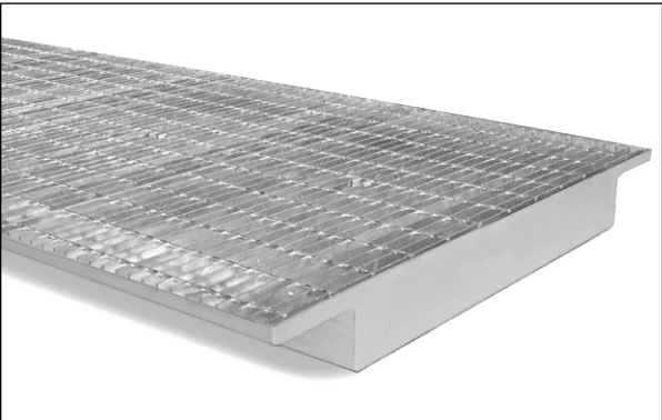
These space-saving Sump Inserts are mounted directly between the cross beams
