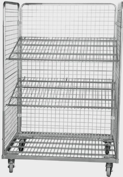
Steel roll box pallet for Euro pallet, 3 mesh walls, 950 x 1350 x 1820 mm, brake, order number 266-088-T1
