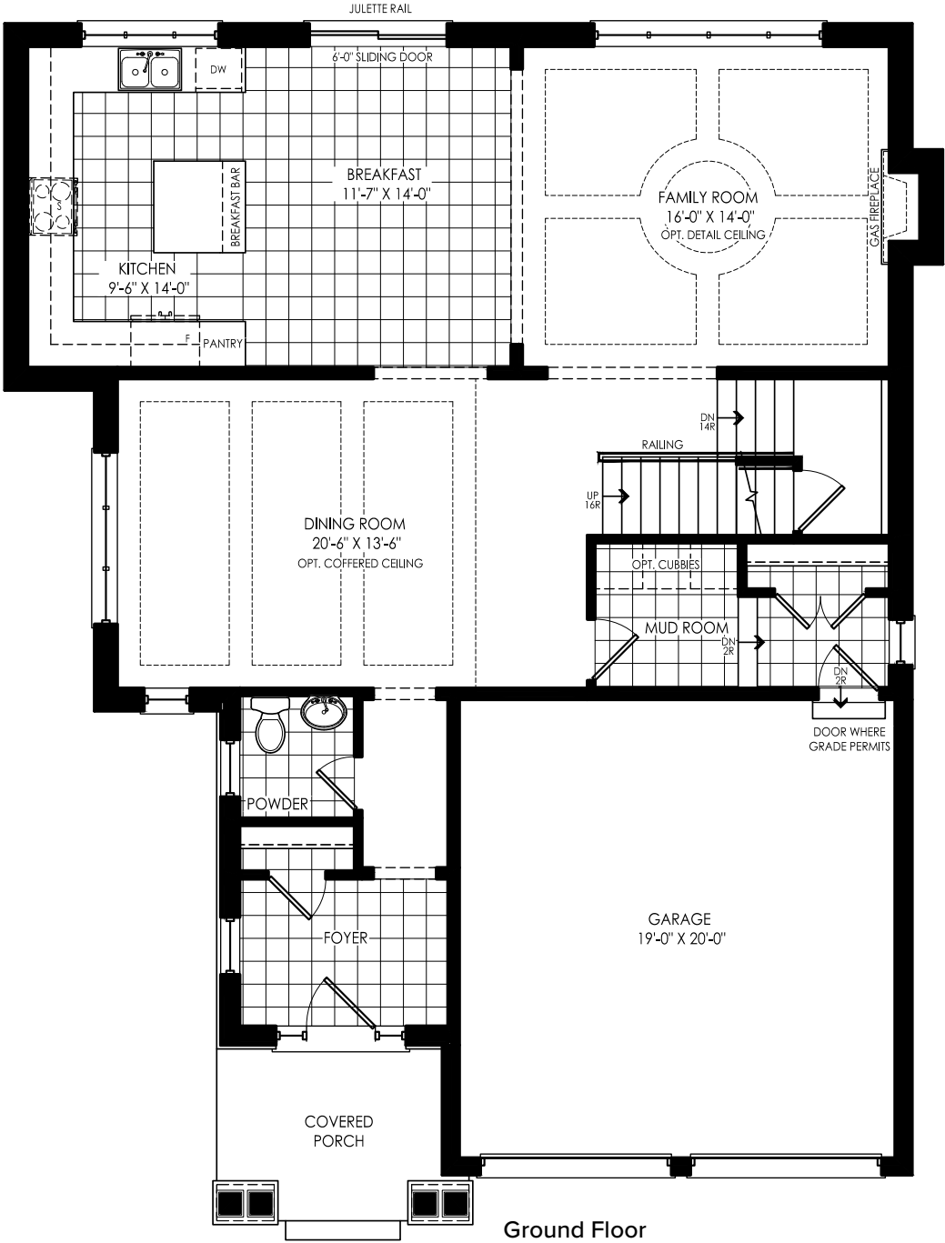
Ground Floor Elev. B
