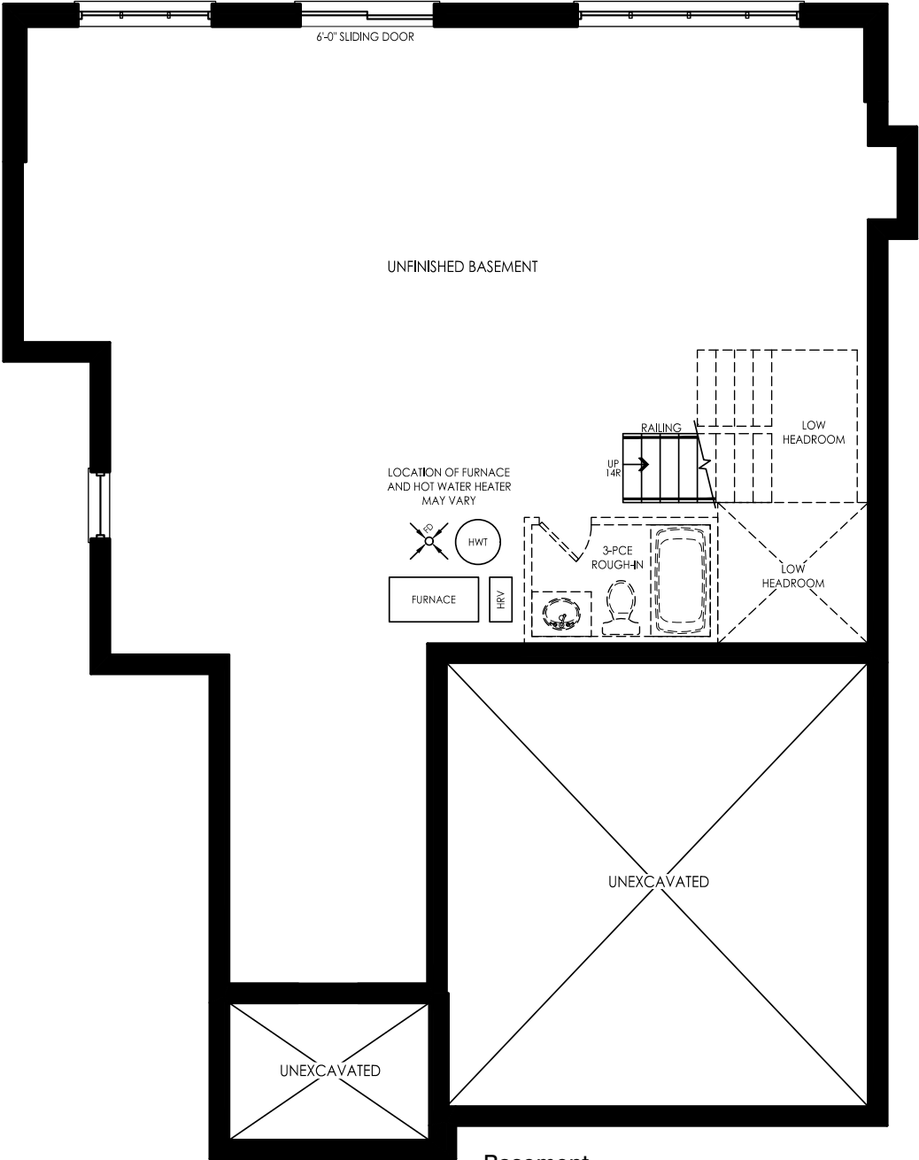
Basement Elev. B
