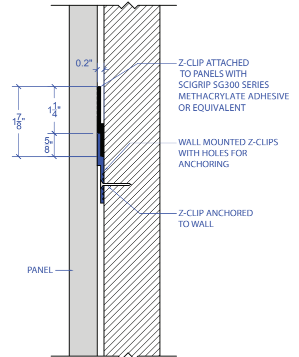
Z-Clips
