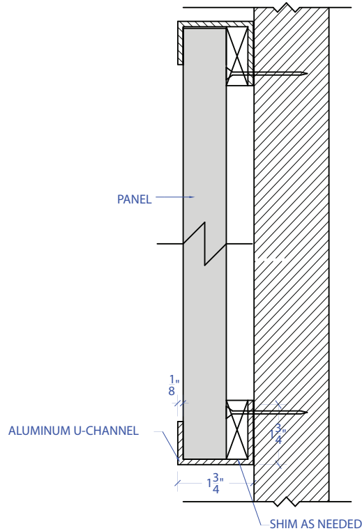
J-Channel
