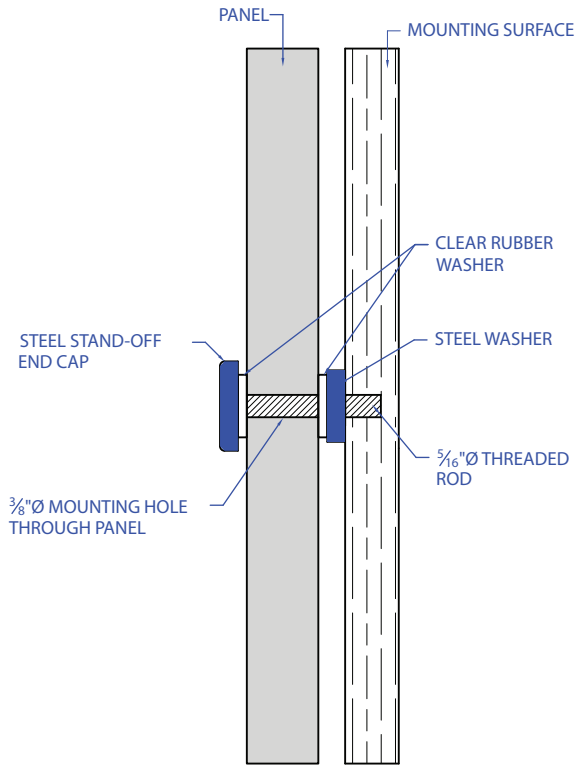
Stand-Off Systems
