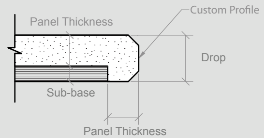
Custom Drop Down Profile Edge
