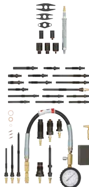
#818010 Master compression test set, 37-pcs
