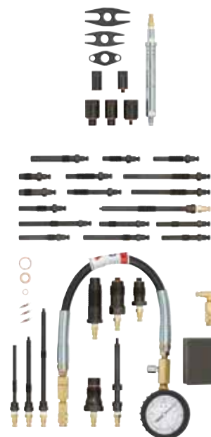
#818010 Compressietestset, 37-dlg.
