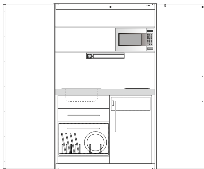
drawing: SKM 120 - Basic model - fully equipped
