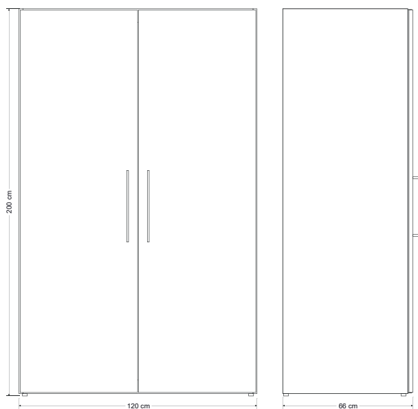
drawing: SKM 120 - measures
