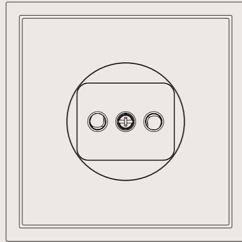
BASE BIPOLAR 2-PIN SOCKET
