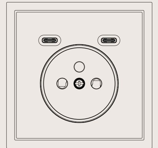
BASE FRANCESA + USB C+C FRENCH SOCKET + USB C+C
