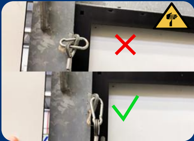
4. Before raising the mast, check that the hooks of the guy wires can move freely in the hole.
