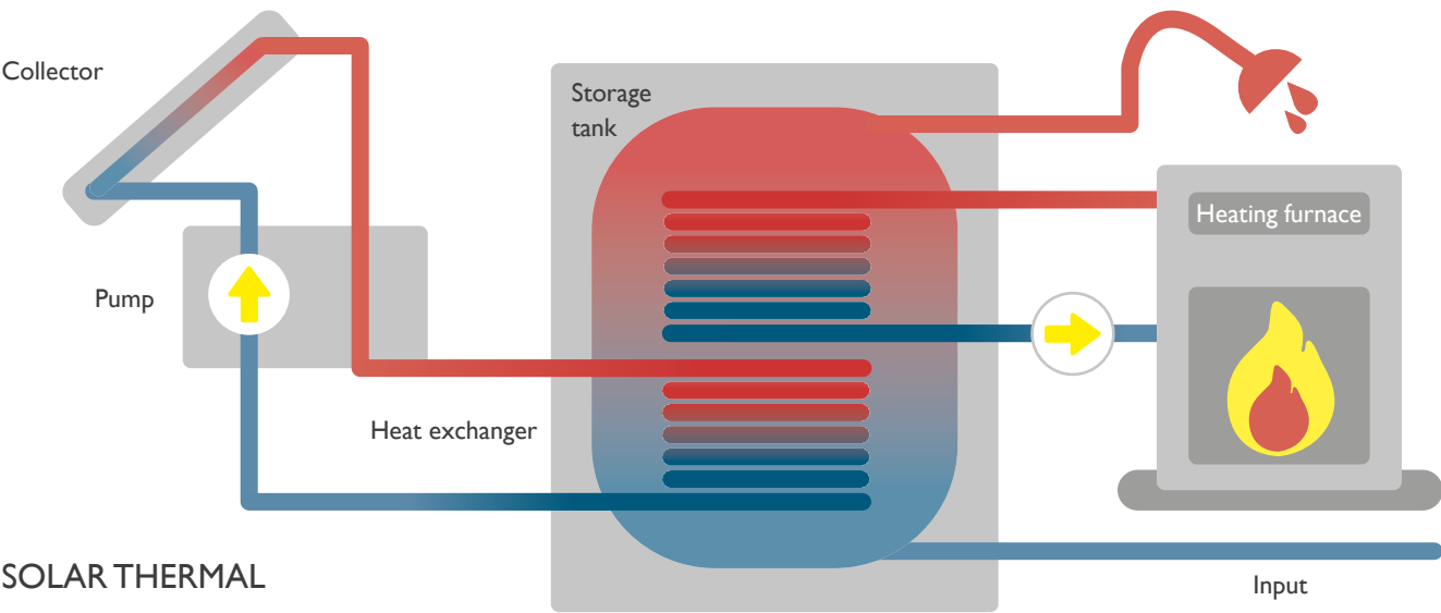
Chart: Solar thermal energy vs. PV system
