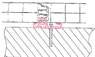
Aluminium Flachsoganker
