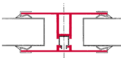
Aluminium H-Sprosse
