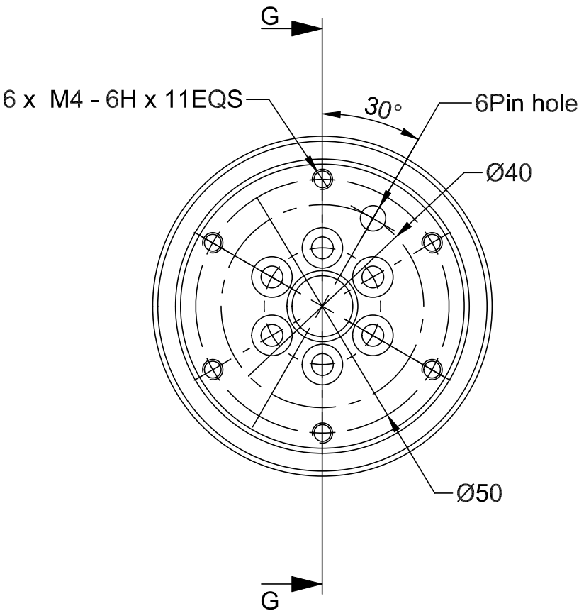
End flange mounting size
