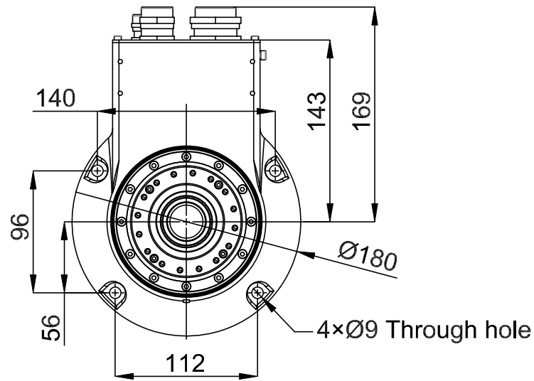
Base mounting size
