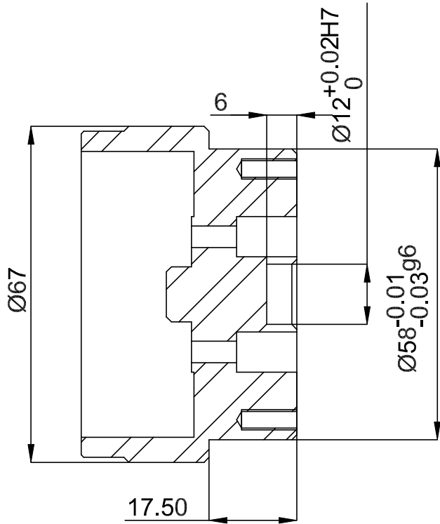
Profile mapG-G Size scale 1 : 1
