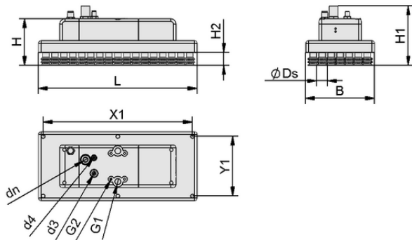
Design data FQE Xc 300x130 SW80 SPB2
