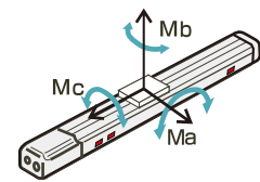
Motor direct mount type
