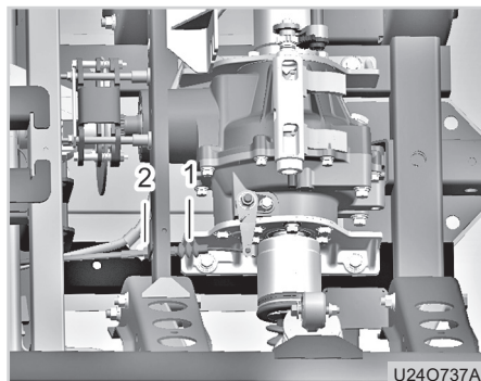
(1) Differentialsperrenkabel (2) Mutter
