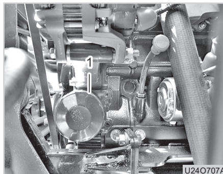
(1) Ölfilter
