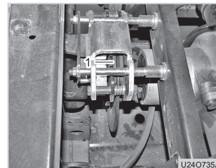
(1) Scheibenbacke
