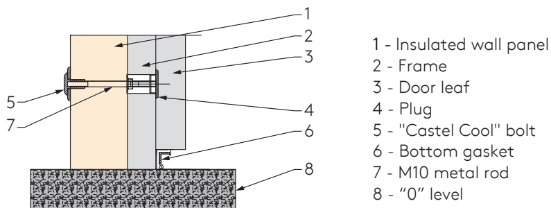
Assembly to insulated wall panel - threshold
