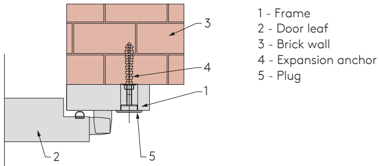
Traditional assembly (brickwall)
