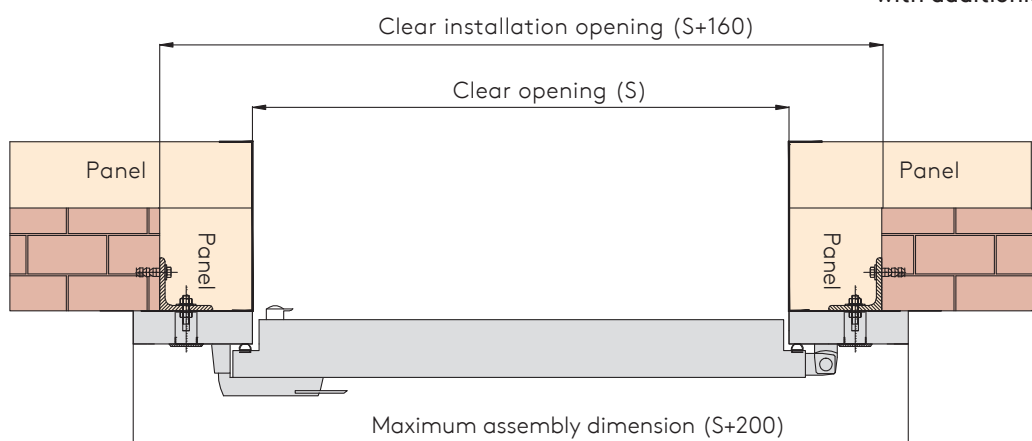
Traditional assembly (brickwall) with additional insulation
