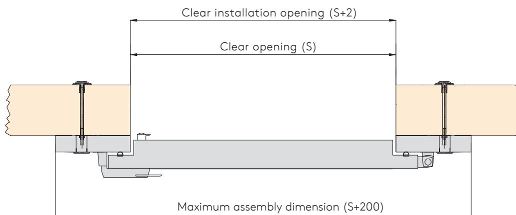
Assembly to insulated wall panel - one frame
