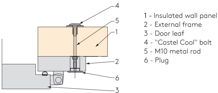
Assembly to insulated wall panel – one frame
