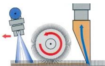
Injection-extraction cleaning
