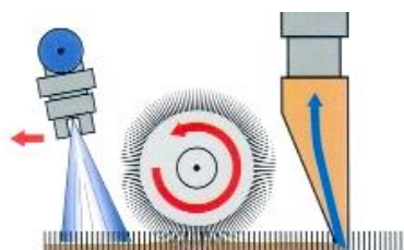
Injection-extraction cleaning with rotating brush
