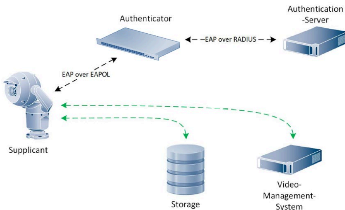
Figure 1: EAP (Extensible Authentication Protocol) data is first encapsulated in EAPOL frames between the Supplicant and Authenticator, then re-encapsulated between the Authenticator and the Authentication Server using RADIUS or Diameter.
