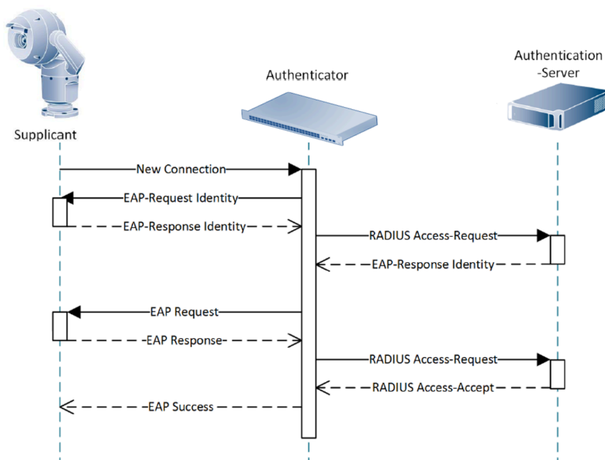
Figure 2: 802.1x Authentication Sequence Diagram
