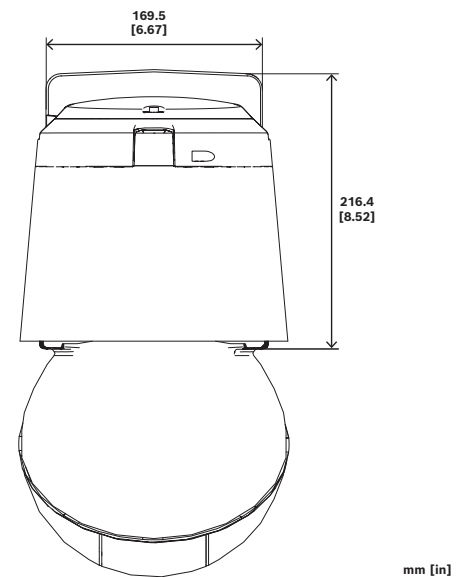
Fig. 2: Dimensions in mm (in.) of the camera on NDA-7100-PEN | NDA-7100-PENF (front view)
