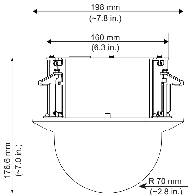
Fig. 1: In-ceiling model
