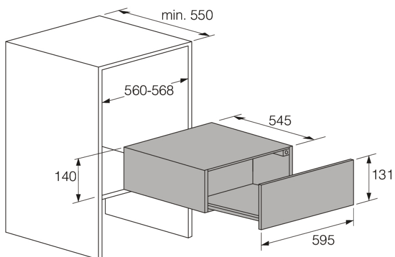
Craft warming drawer (old)
