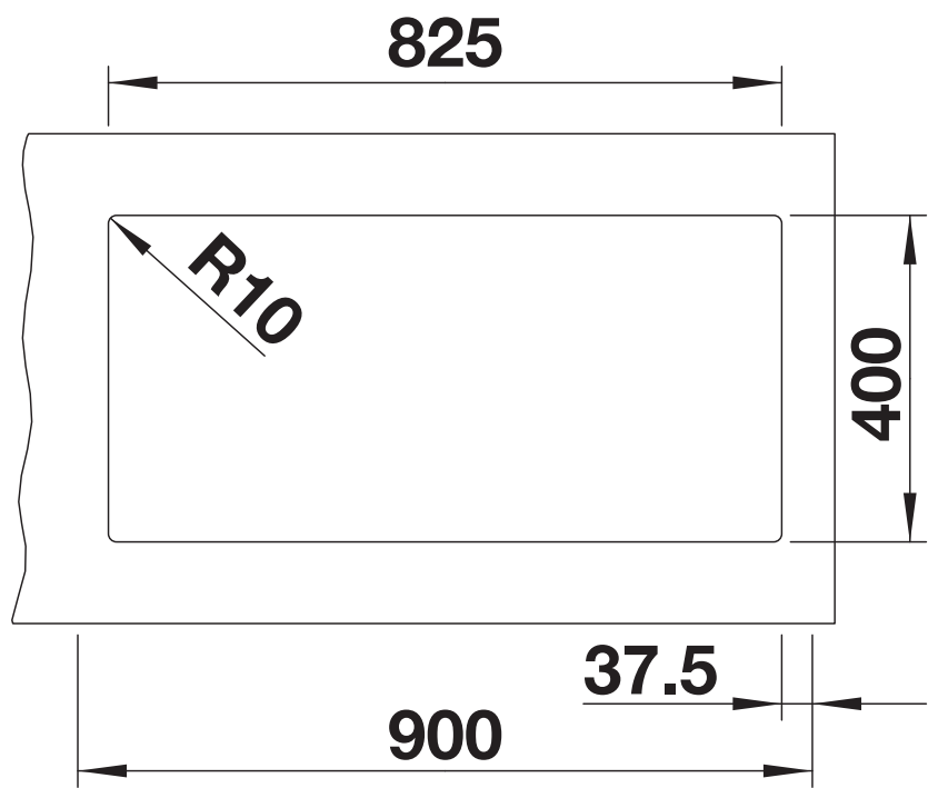
Cut-out
