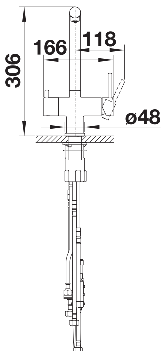
Side view lever
