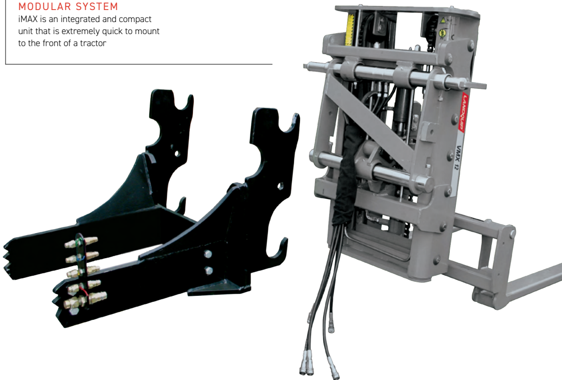
Front mount with tilt only
