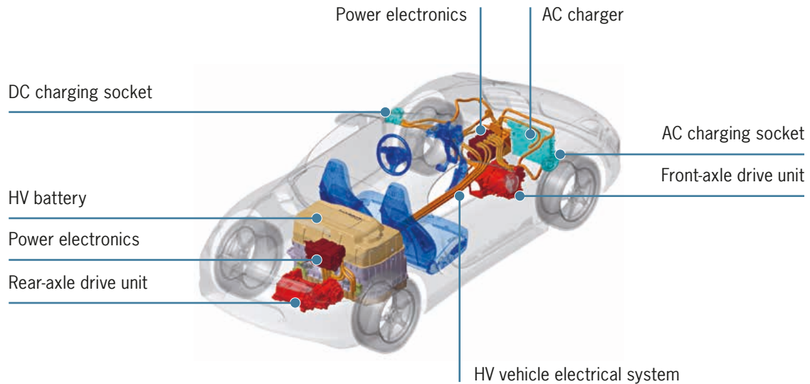
Overview of high-voltage components in the vehicle
