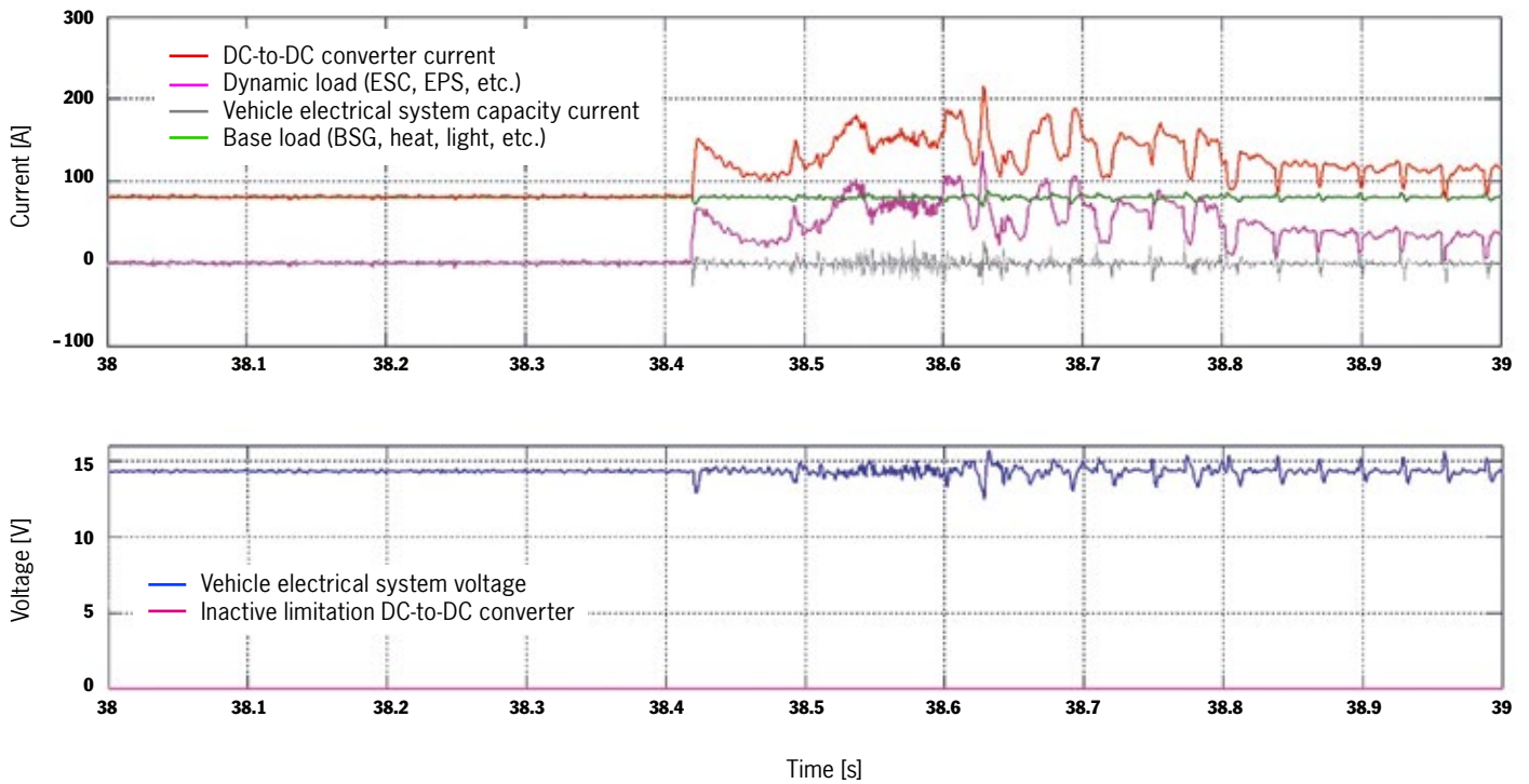
Figure 5: Current profile in the vehicle electrical system with a 3-kW DC-to-DC converter
