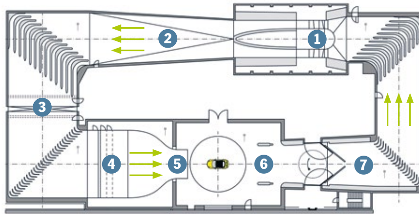
Structure of the new aeroacoustic wind tunnel
