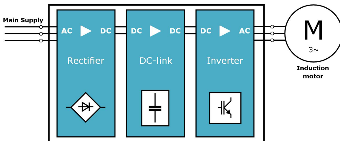
Figure 2: Energy conversion process using a variable frequency drive
