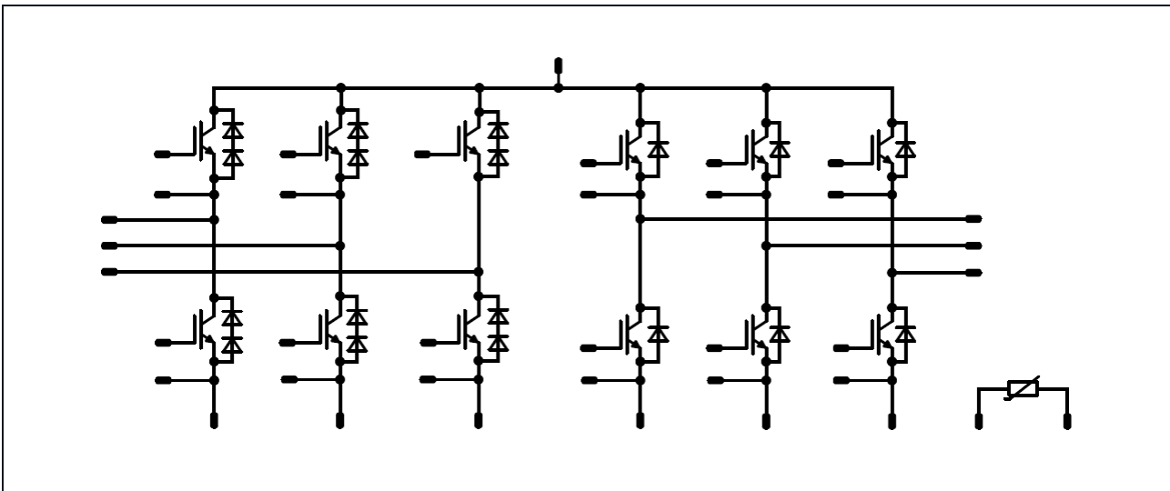
Figure 6: Twin-pack with tandem diode
