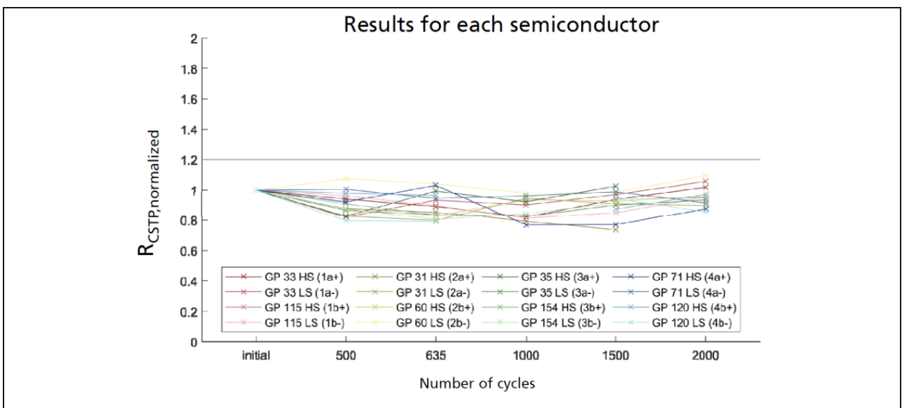
Figure 5: Normalized R_{th}(j-s) of flow S3 at passive temperature cycling ( -40 °C/ +125 °C, test stopped at 2k cycles)
