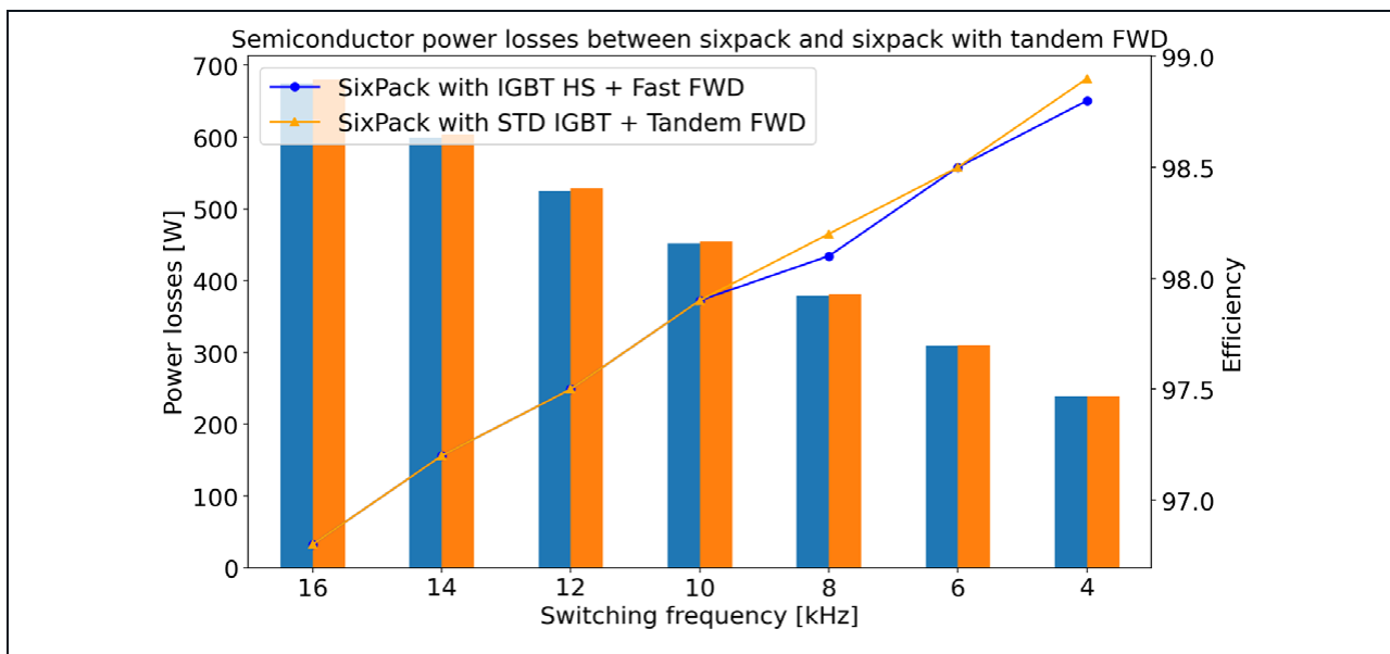
Figure 5: Power losses and efficiency results comparing the sixpack topology with (high speed) HS IGBT technology against the standard IGBT with tandem diode implementation
