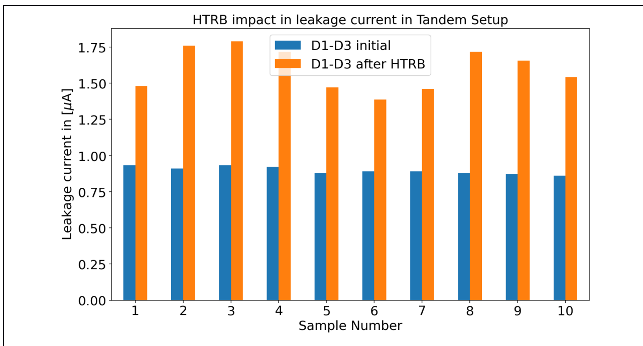
Figure 12: Measurement of the reverse leakage current of the tandem diode configuration before and after HTRB using diodes with high and low reverse leakage current
