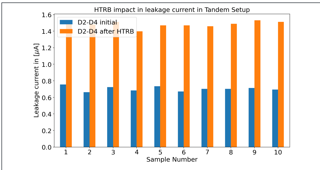
Figure 13: Measurement of the reverse leakage current of the tandem diode configuration before and after HTRB using diodes with average reverse leakage current
