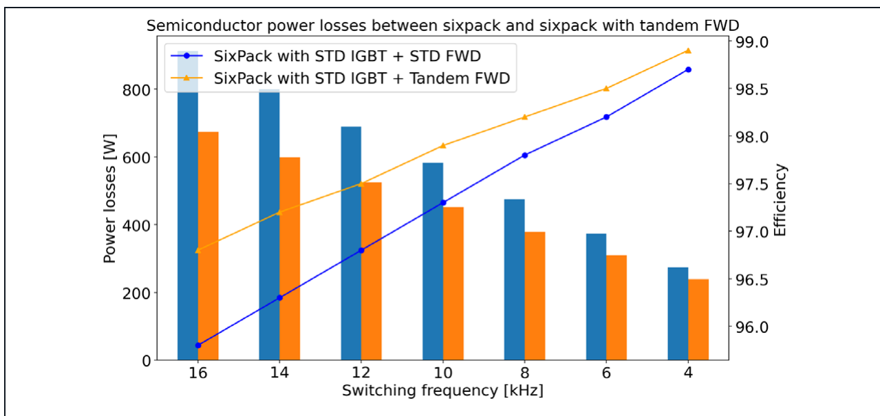
Figure 4: Power losses and efficiency results comparing the standard sixpack topology against the tandem diode implementation
