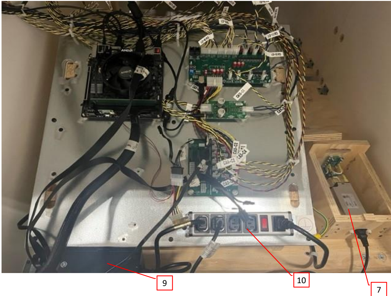
Photo 2- Main Cabinet
