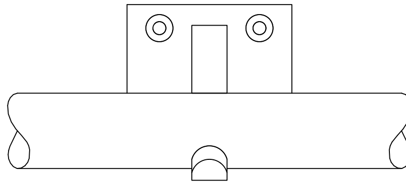
Classic French return double pole centre passing bracket - Front View
