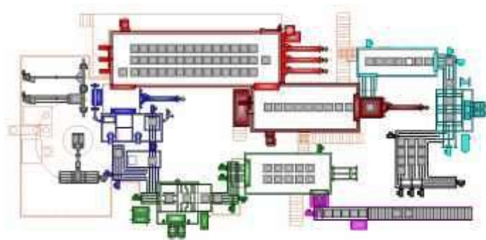
4.3 Three-lined pusher type plant with possibility for the parts withdrawal for press hardening
