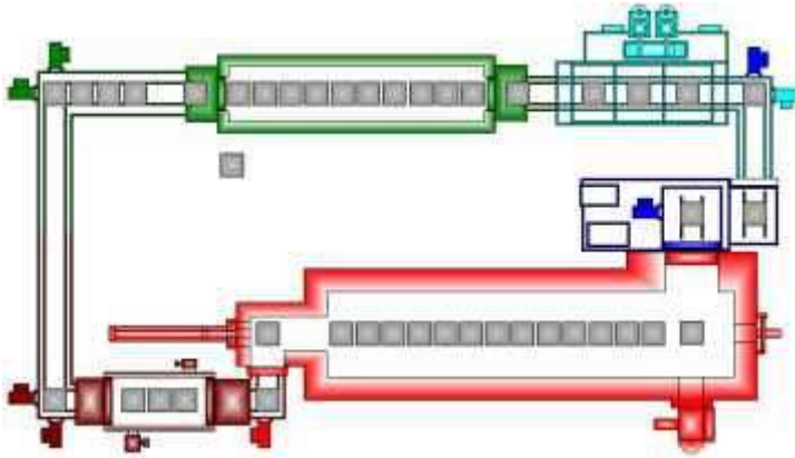
4.1 Single-lined pusher type furnace plant for carbonitriding
