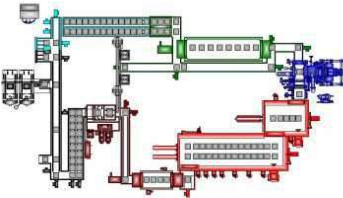
4.2 Two-lined pusher type plant with separate diffusion chamber and high pressure gas quenching
