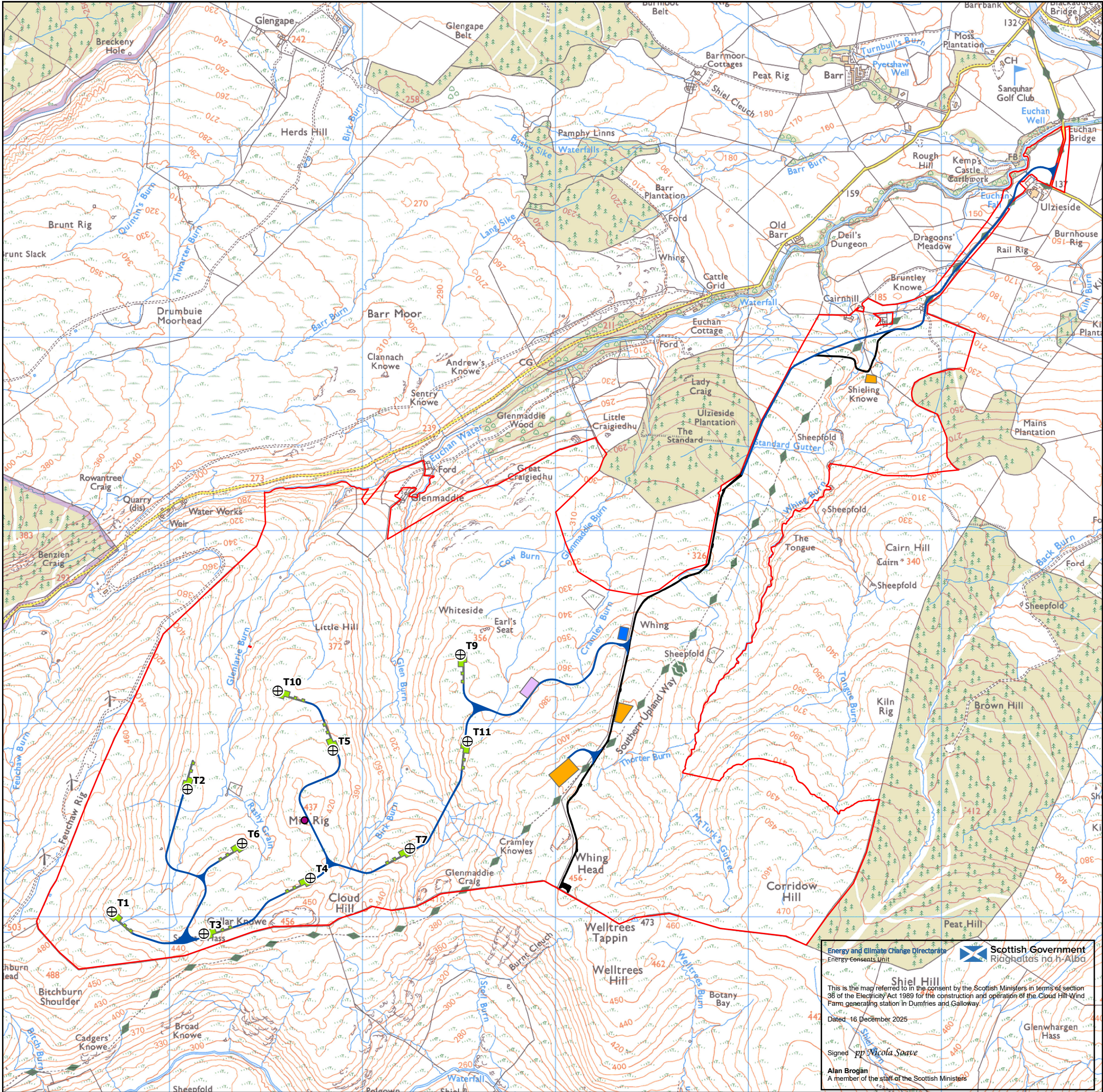
FIGURE 1.2B: Amended Revised Development Site Layout
