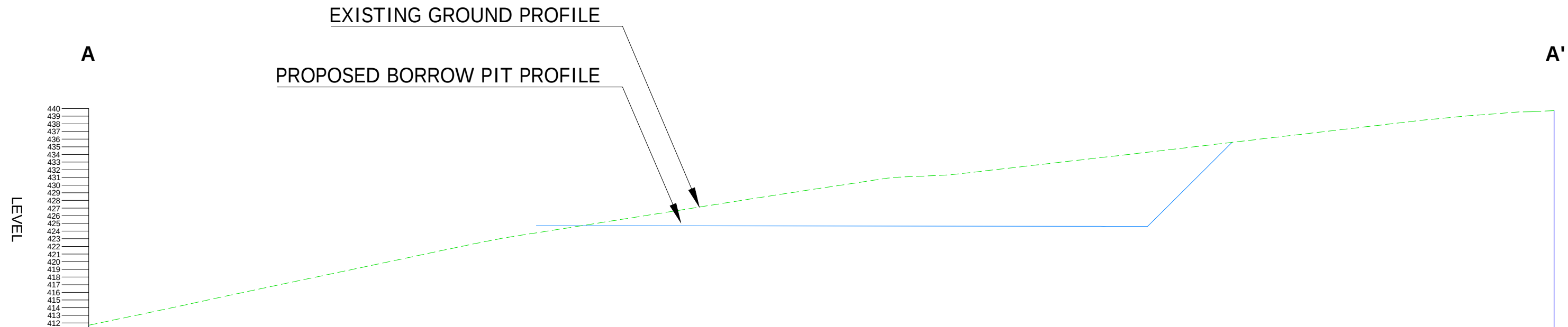
BORROW PIT (c) SECTION A-A' SCALE H 1:500, V 1:500. DATUM 411.000
