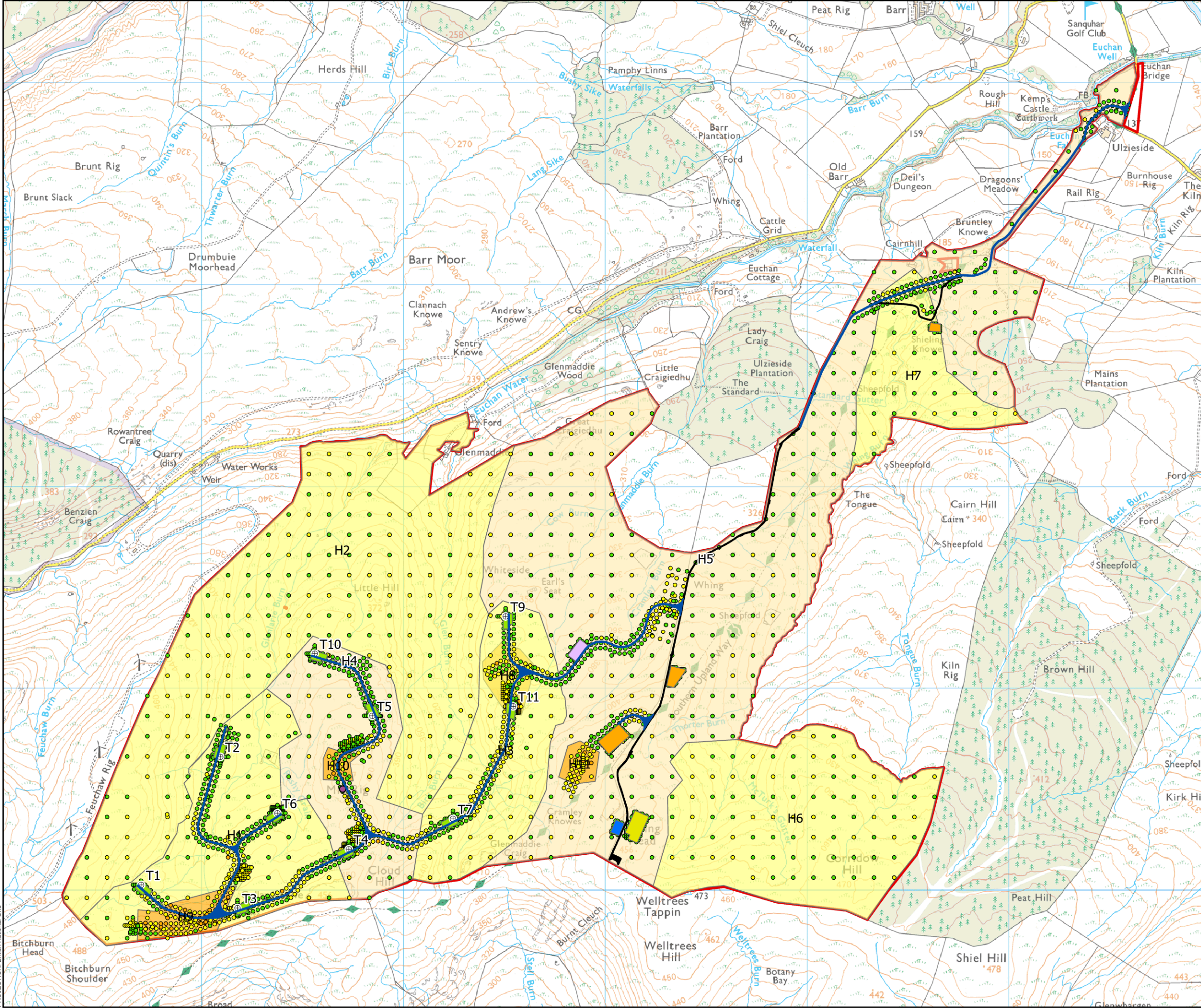
Figure 10.1.7 Hazard Ranking Zonation Plan Cloud Hill Windfarm Peat Slide Risk Assessment
