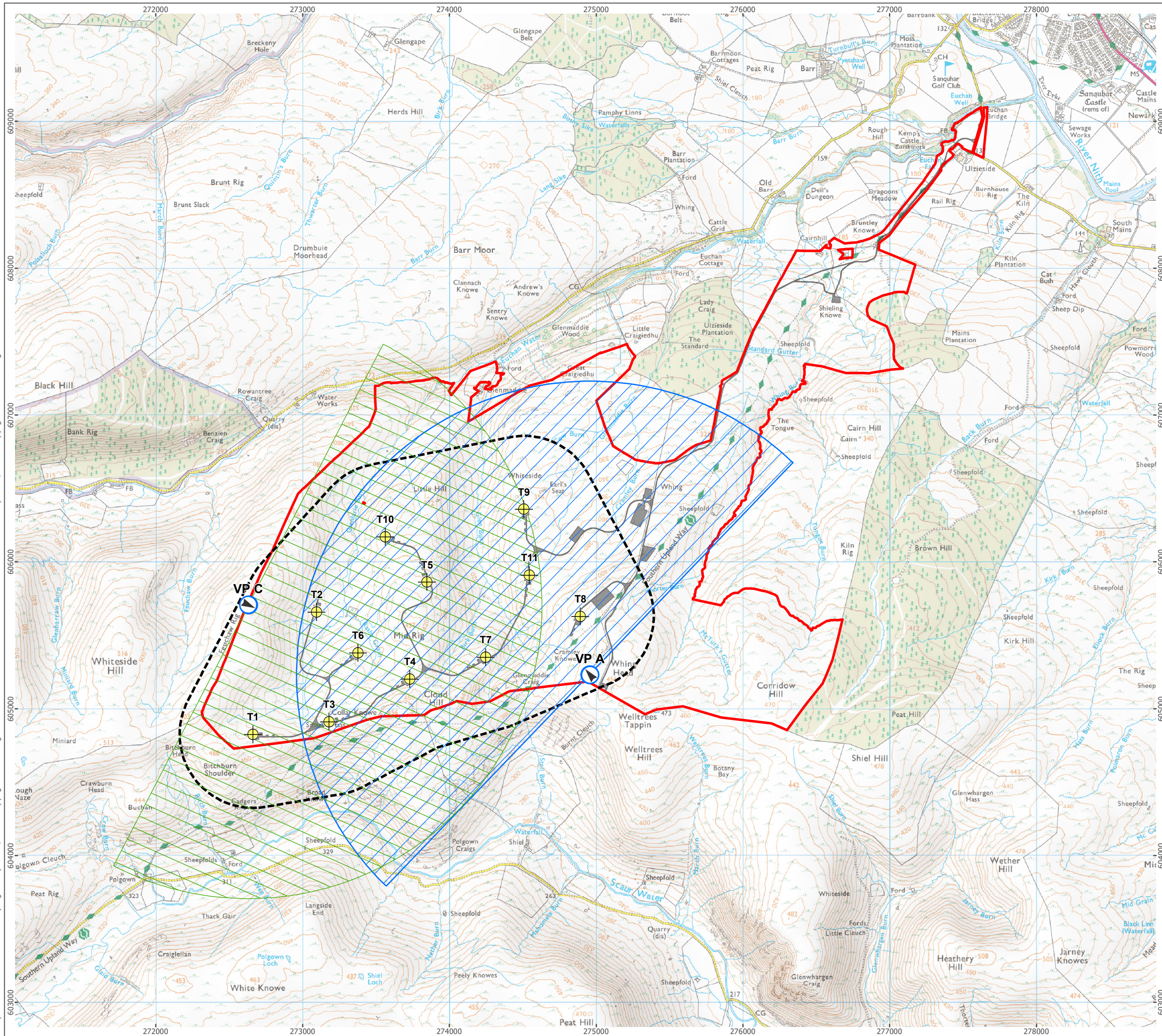
Vantage Points and Viewsheds Figure 8.1 Cloud Hill Wind Farm EIA
