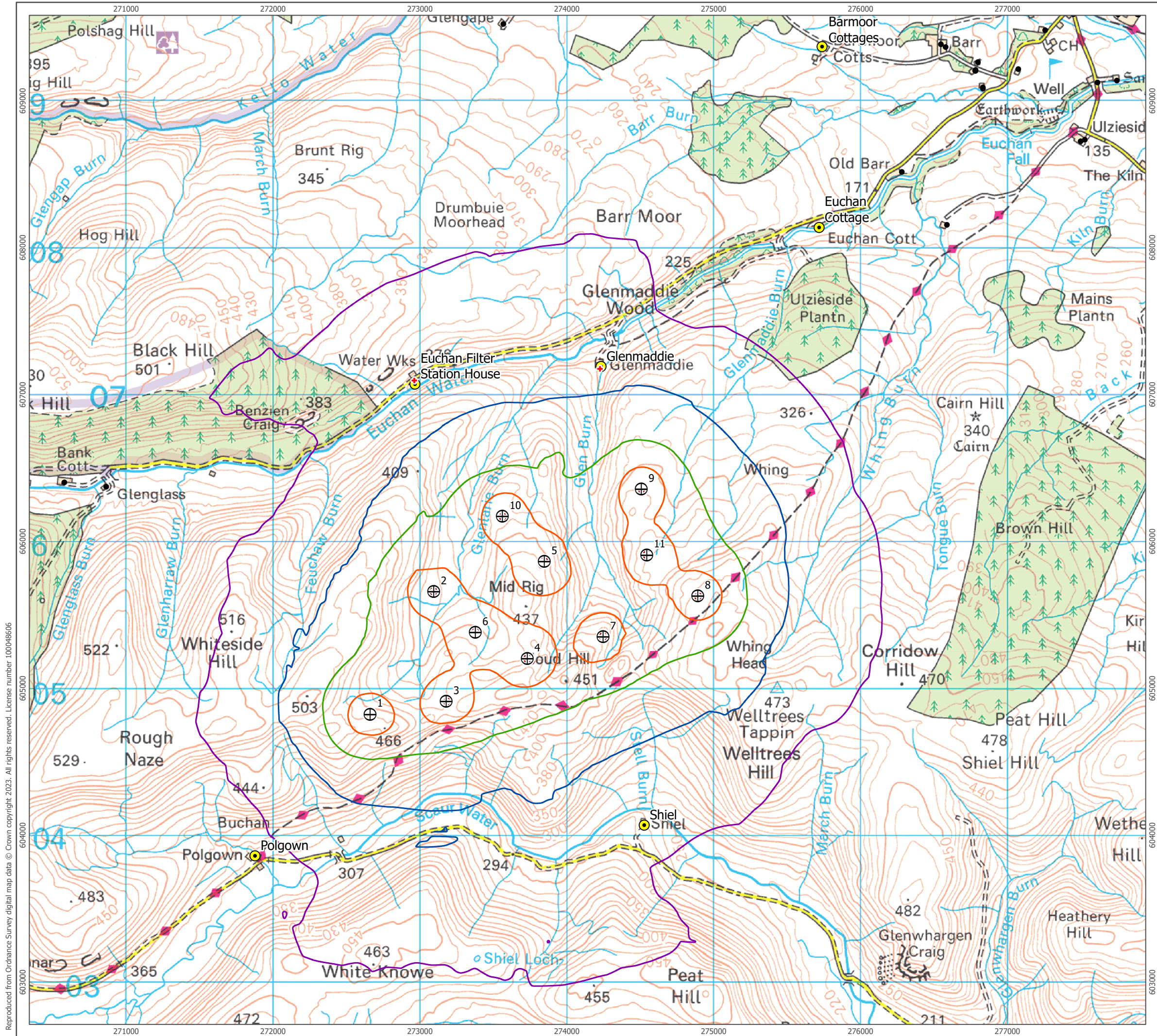
Noise Contour Plot Figure 12.3 Cloud Hill Wind Farm EIA
