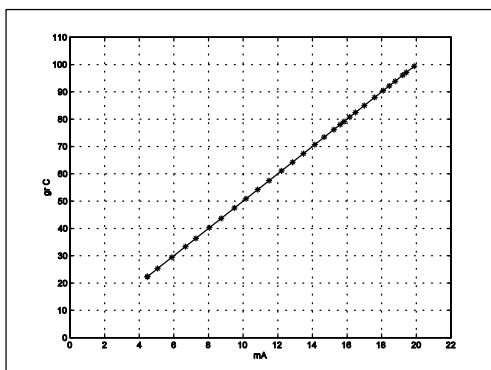
Typ. linearity
