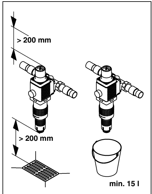
Simipur Master 1½" - 2"
