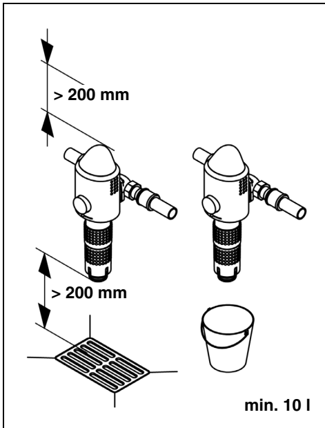
Simipur Master 1" - 1¼"
