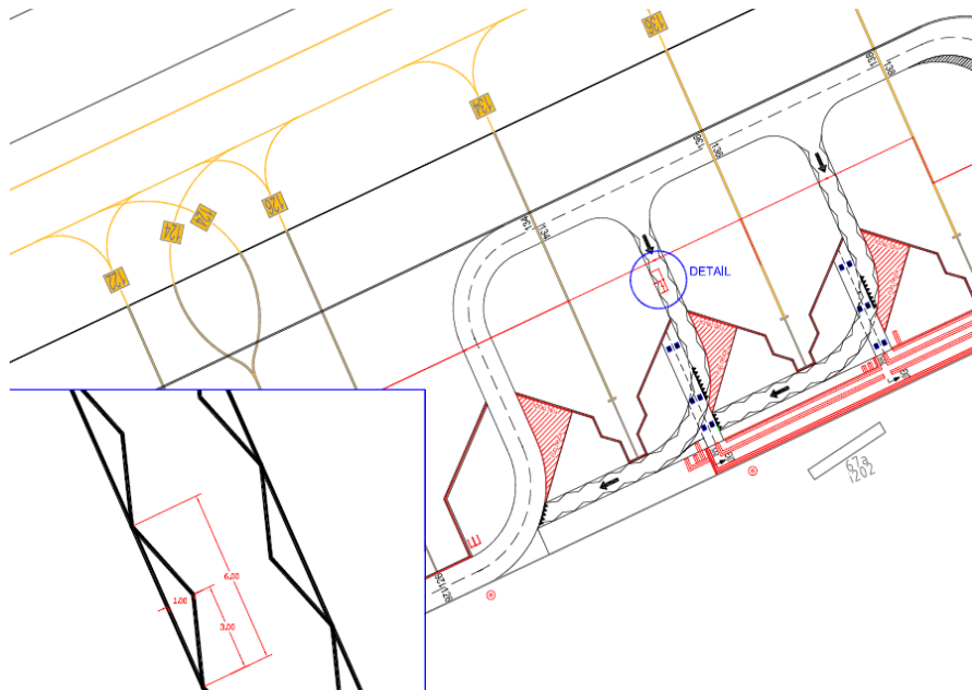
Fig. 20. Aircraft stand service drive
