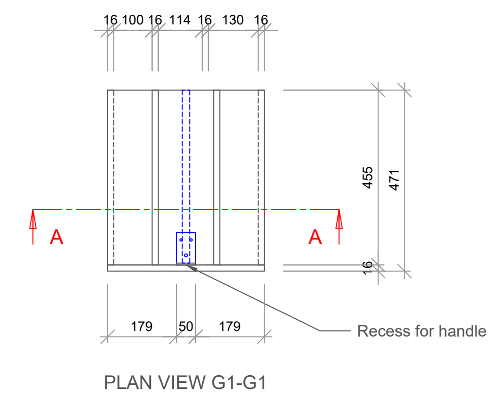
PLAN VIEW G1-G1
