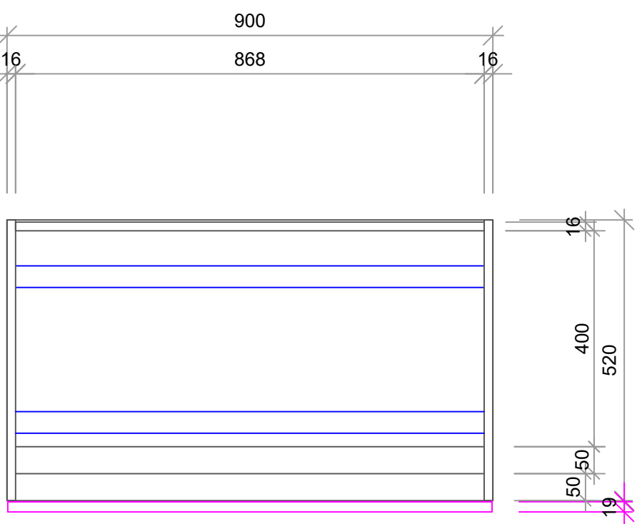
VIEW SECTION
