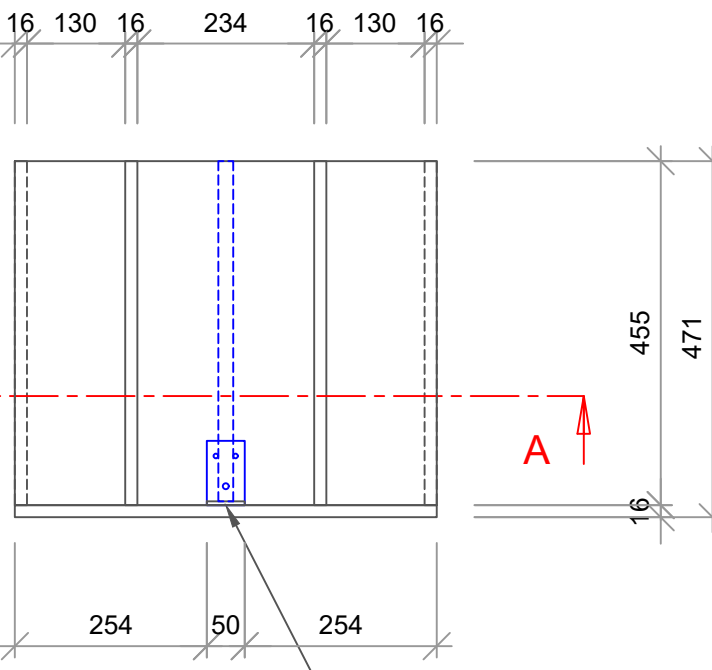
PLAN VIEW G1-G1
