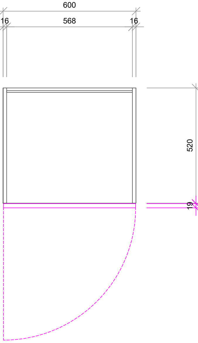
PLAN VIEW G1-G1
