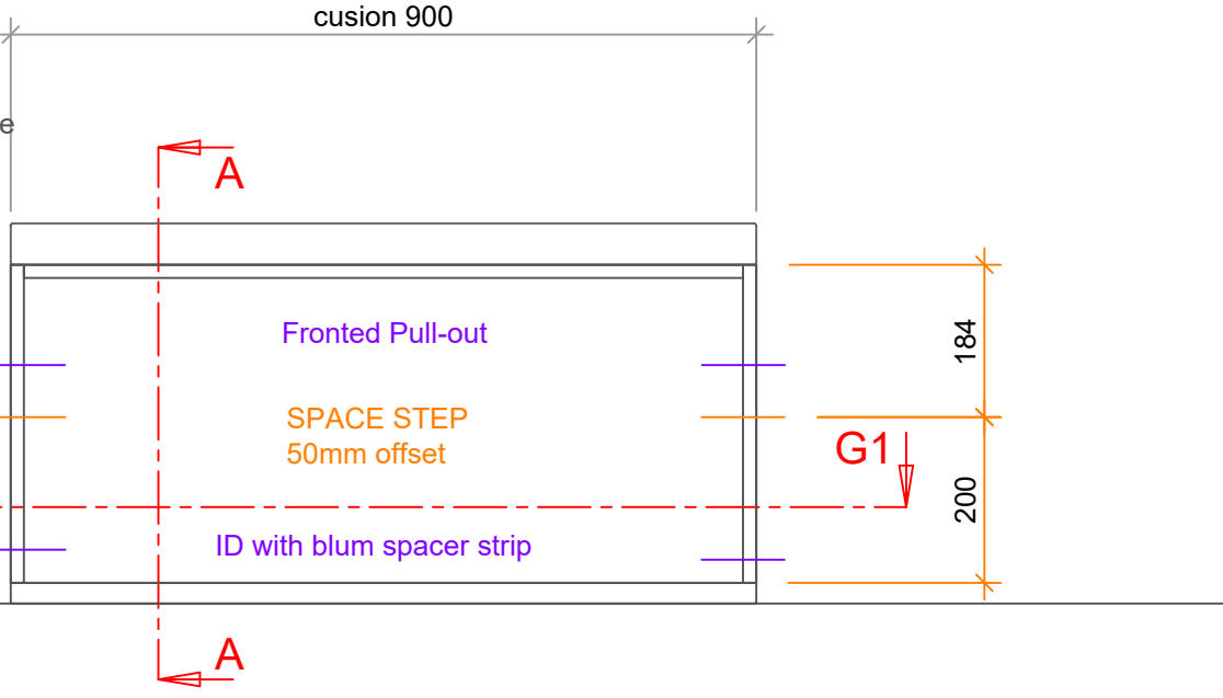
VIEW SECTION
