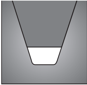
Correct belt arrangement in the V-grooved pulley
