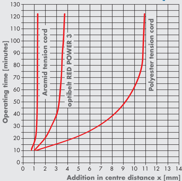
Test arrangement centre distance increase [mm]
