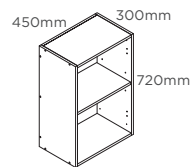
450mm wall cabinet
